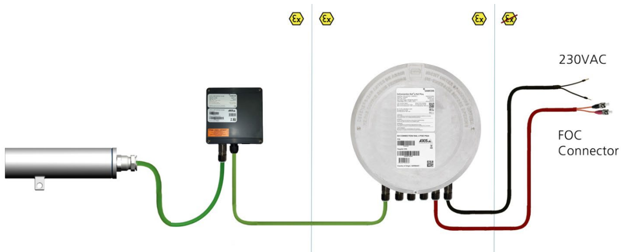
Fig. 5-9 ExTB-2 -> ExConnection Rail
