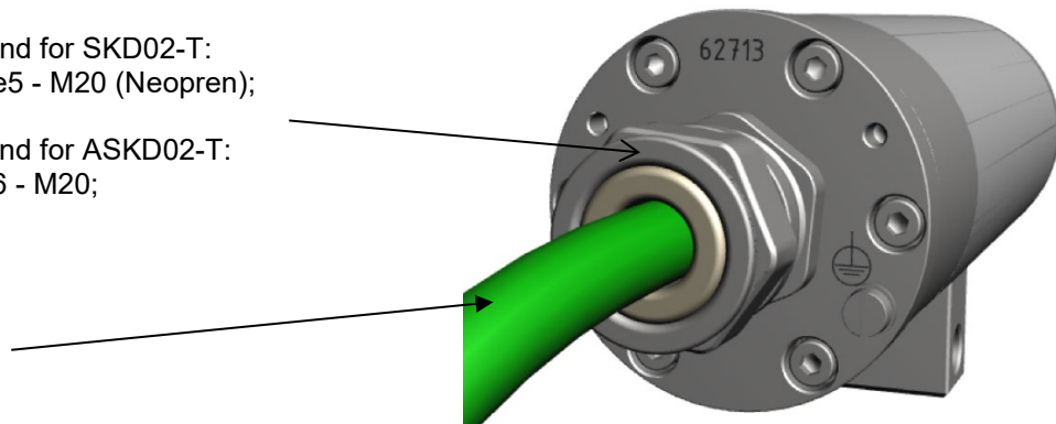
Fig. 5-2 Ex-d Cable gland and cable
