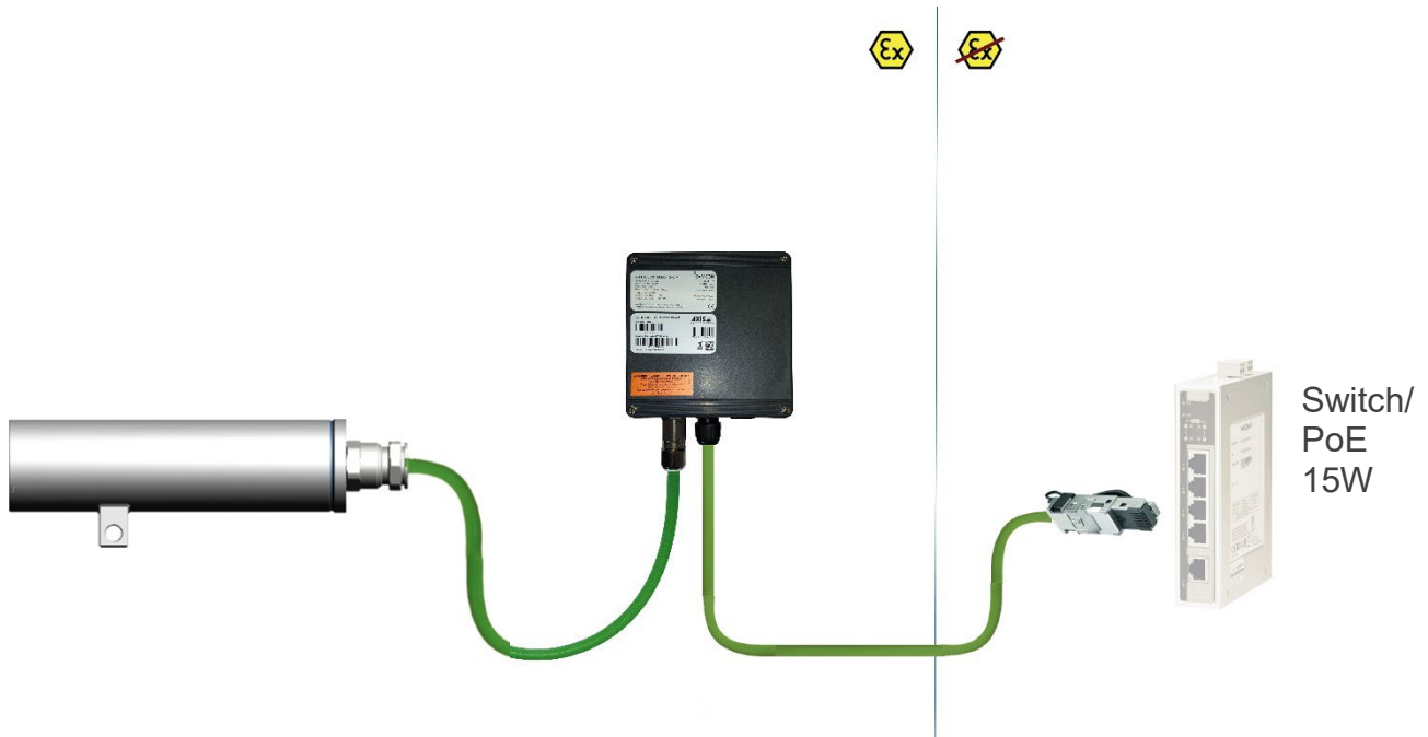
Fig. 5-8 ExTB-3 -> Safe area
