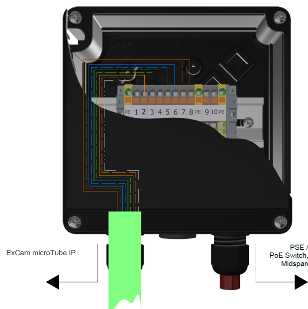
Fig. 5-6 Sample circuit of terminal box ExTB-2
