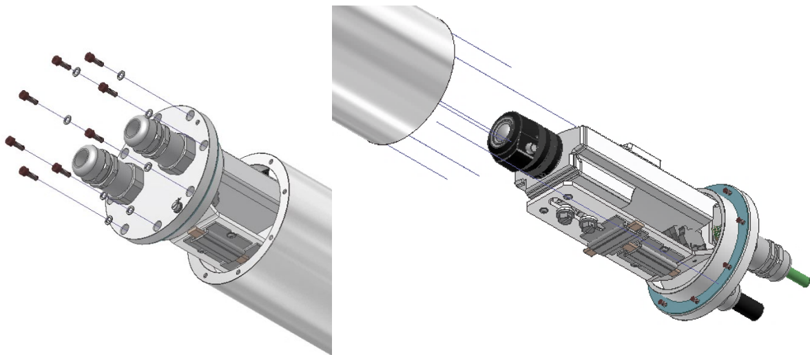
Fig. 6-3 Opening the RoughCam IPQ1656 (similar illustration)
