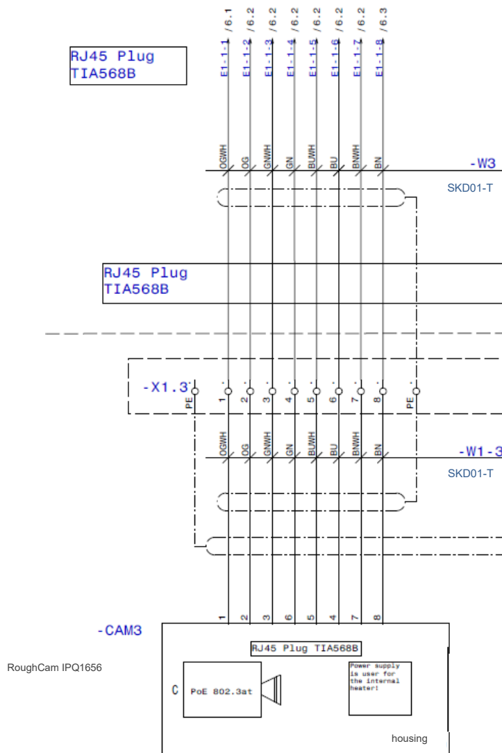
Fig. 5-8 Sample circuit of terminal box (without heater)
