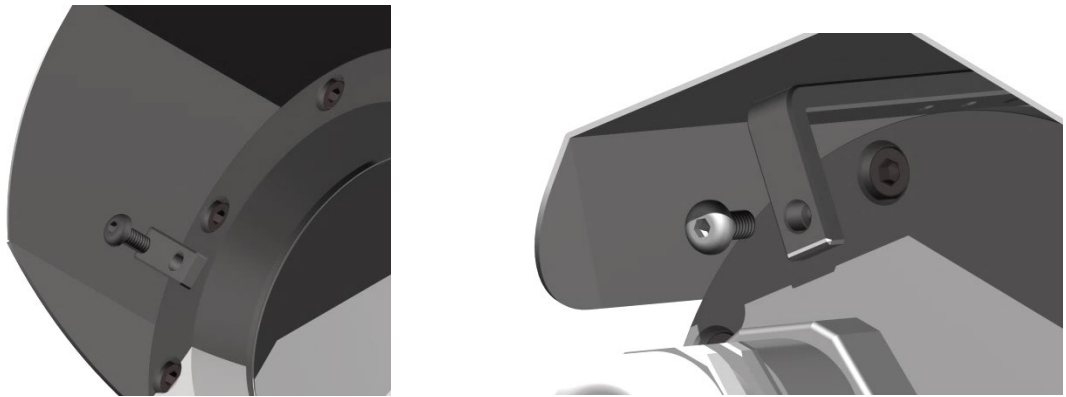
Fig. 6-1 Removing the weather protection roof (1/2) (similar illustration)
