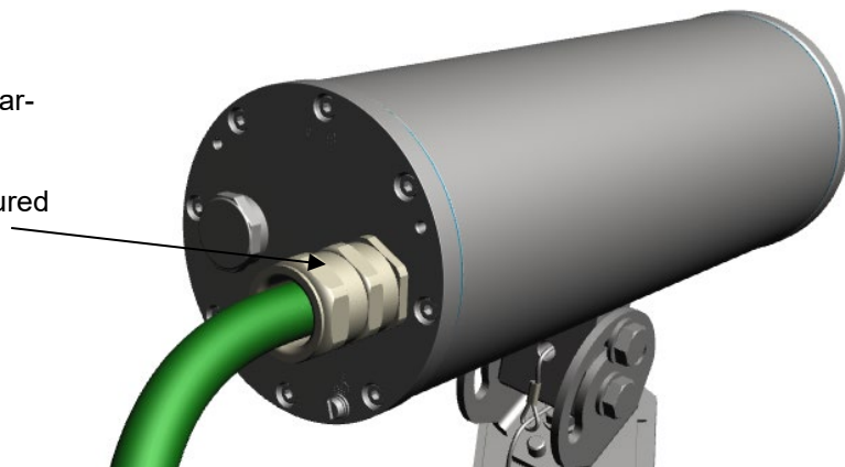
Fig. 5-2. Cable gland and supply line
