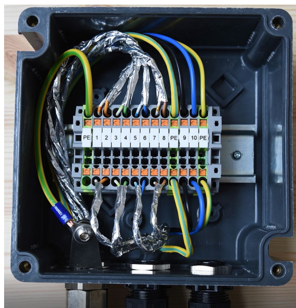
Fig. 5-9 Sample circuit of terminal box (heater integrated)
