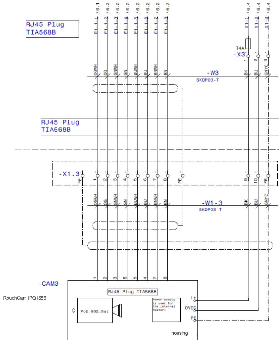
Fig. 5-9 Sample circuit of terminal box (heater integrated)
