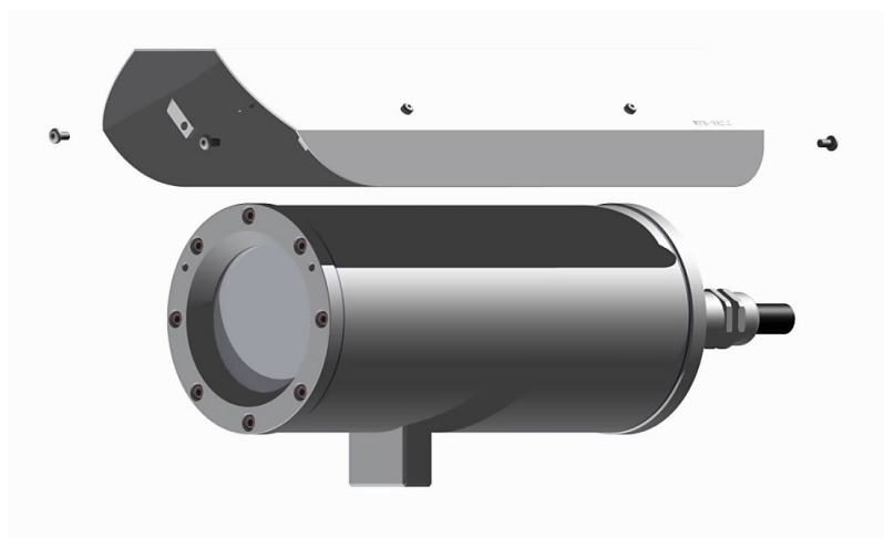
Fig. 6-2 Removing the weather protection roof (2/2) (similar illustration)
