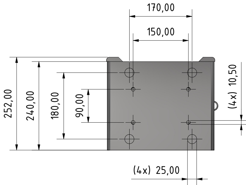
TNXCD housing
