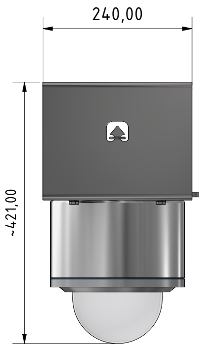
VA4 housing
